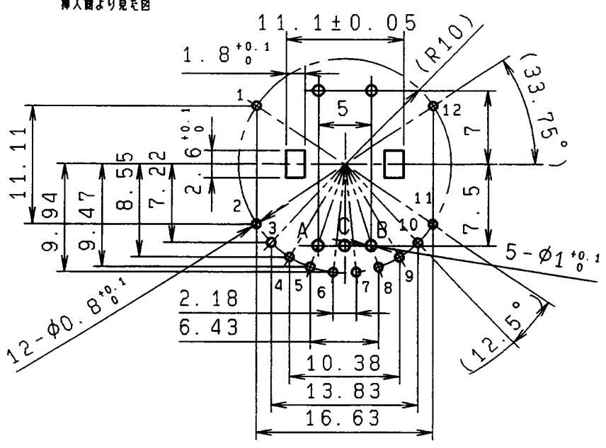
VIEWED FROM MOUNTING SIDE 挿入側より見た図
